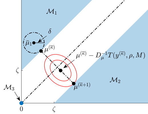
Fig. 5. Domain \mathcal{M} of the Lagrange multipliers associated to the coupling constraints, for the case m = 2 . Notice the minimum distance \zeta between any two subdomains of \mathcal{M} involves the origin as one of these subdomains.
